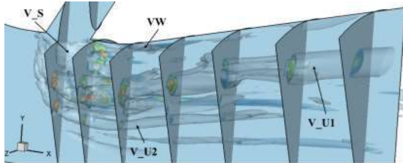
Figure 2 Vortex structure in reverse injection
